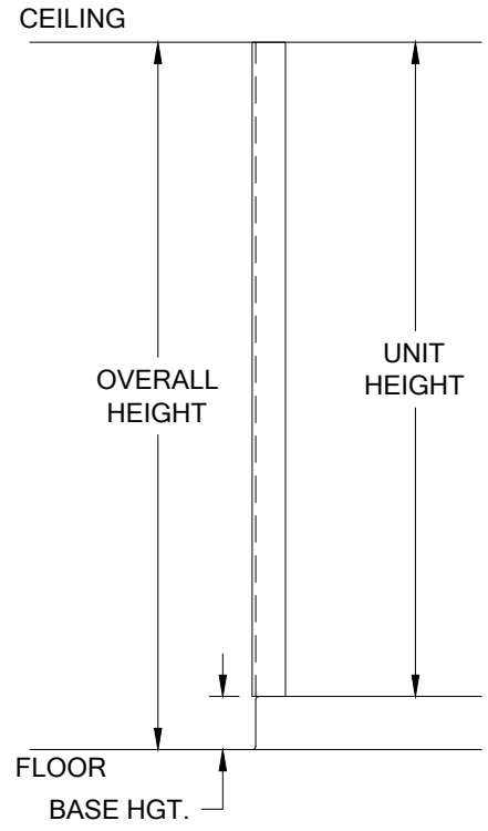
VA-034N CORNER GUARD AT FULL HEIGHT ELEVATION
